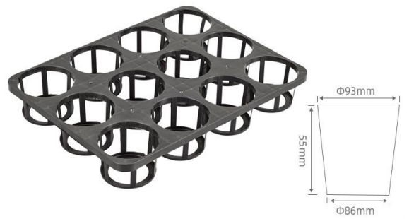
LTHZ12 L42.5*W31.5*H5.5cm
