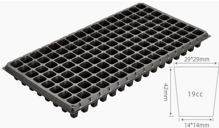
LXQB128A L54*W28*H4.2cm
