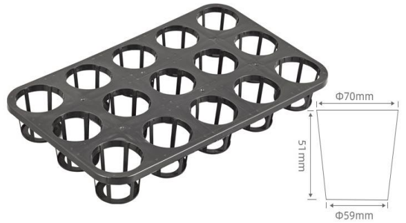
LTHZ15 L45*W27*H5.1cm
