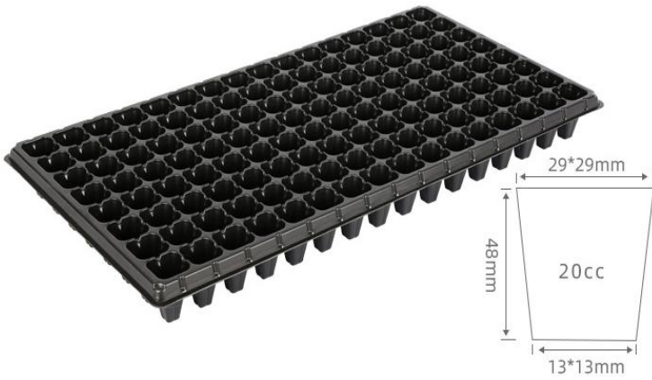
LXQB128 L53.8*W27.8*H4.8cm
